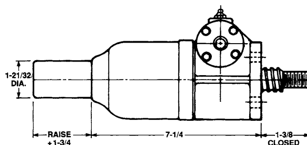
Inverted: M-28002
