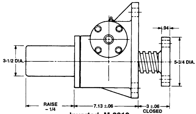
Inverted: M-9019
