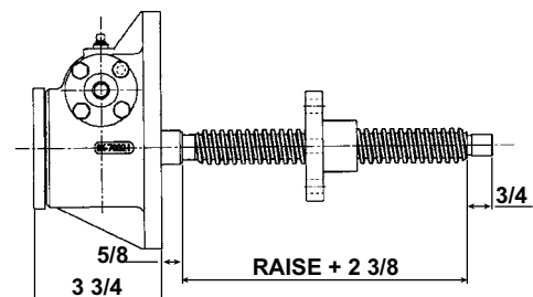
Inverted Rotating: DM-7003
