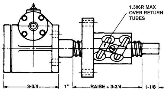
Inverted Rotating: KDM-28004
