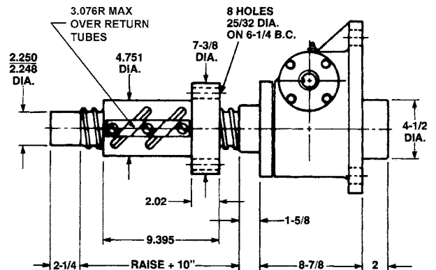
Upright Rotating: UM-9826
