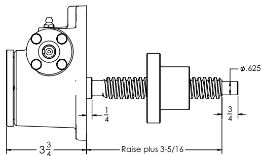
Inverted Rotating: B9003D
