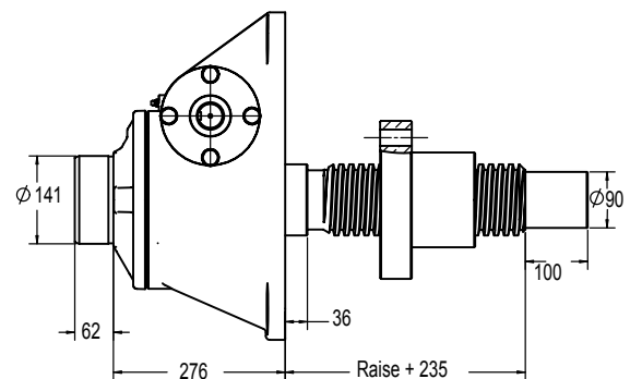
Inverted Rotating: GD9051
