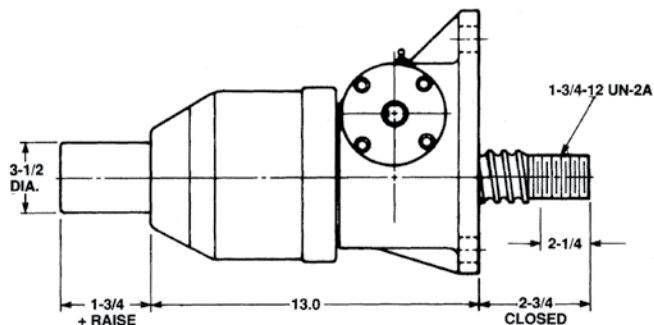
Inverted: M-9819 or M-98191
