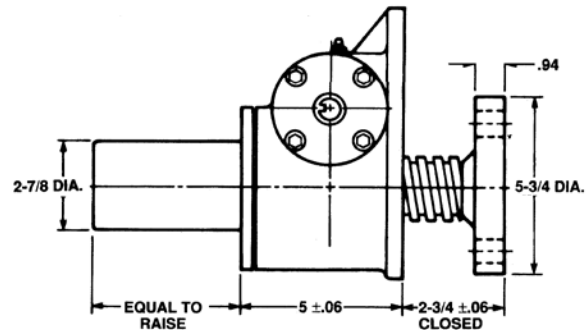
Inverted: M-9009
