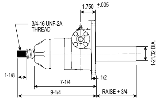
Upright: M-98003
