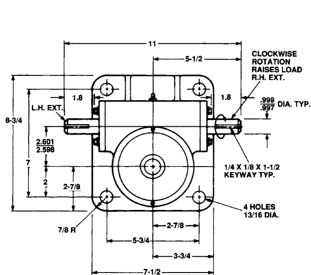
1 1/2" Diameter x 1.000 Lead Lifting Screws
