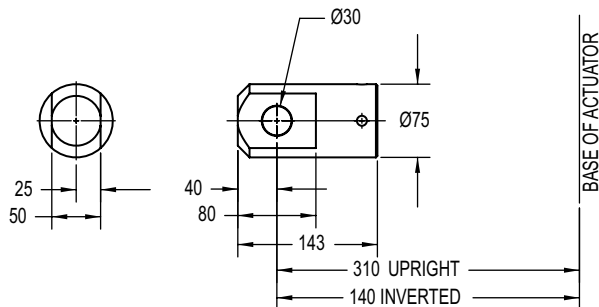
Top Plate G9015-6
