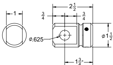
Clevis End SK90003-18A
