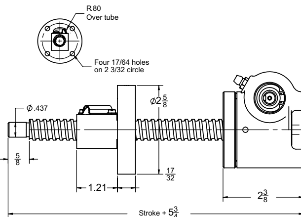
Upright Rotating: B9863U
