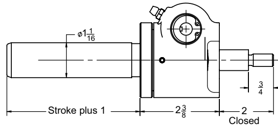
Inverted: B9225TV
