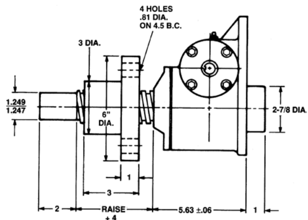
Upright Rotating: UM-9011
