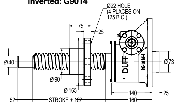
Upright Rotating: GU9016
