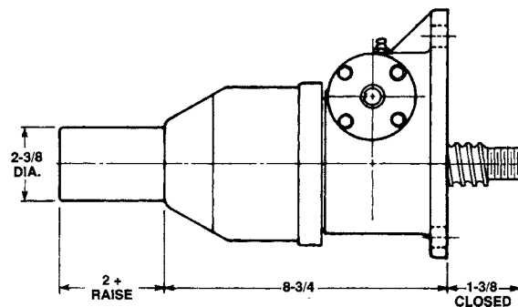
Inverted: M-9804
