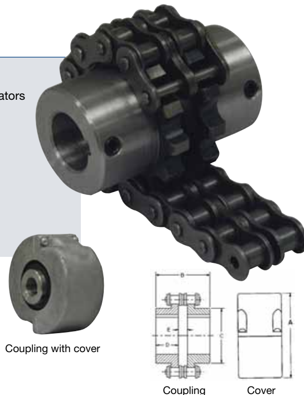
Coupling
