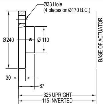
Top Plate G9030-6
