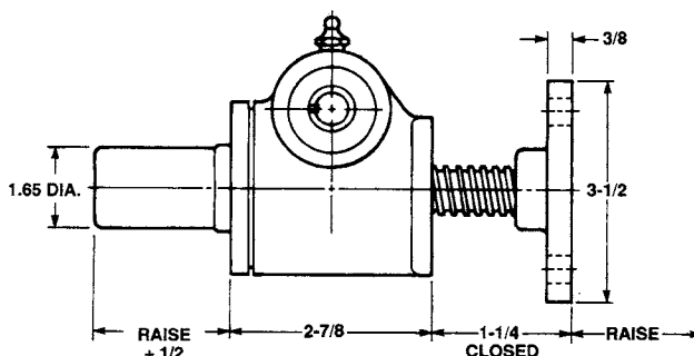
Inverted: M-2500
