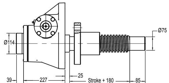
Inverted Rotating: GD9031
