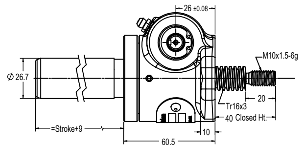
Inverted: G2624
