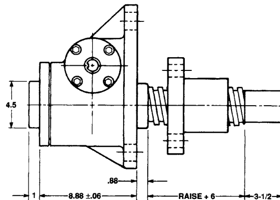
Inverted Rotating: DM-9036
