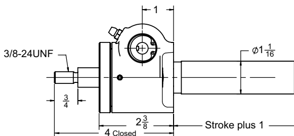
Upright: B9250T
