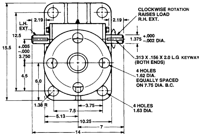
3 3/4" Diameter x .666 Lead Lifting Screws
