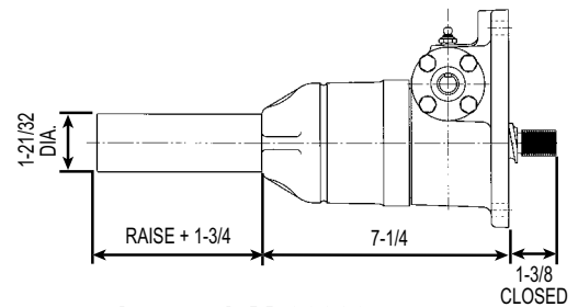
Inverted: M-98002
