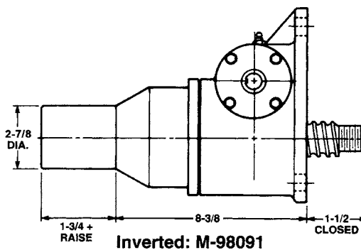
Inverted: M-98091
