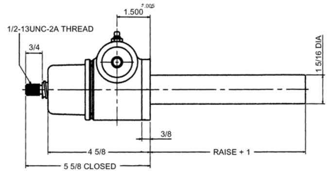
Upright: M-28750
