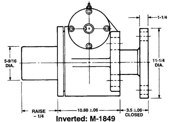
Inverted: M-1849
