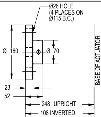
Top Plate G9015-6
