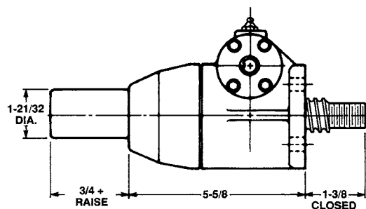
Upright: M-2802
