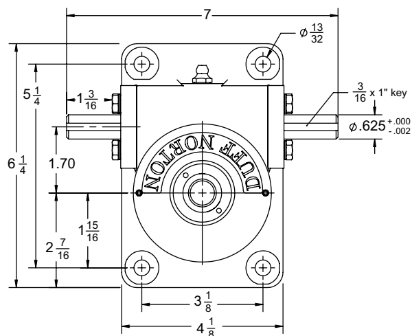
Top View: B9003 1" Diameter x .250"
