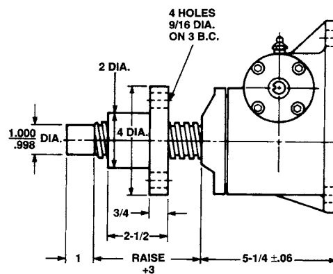
Upright Rotating: UM-9006
