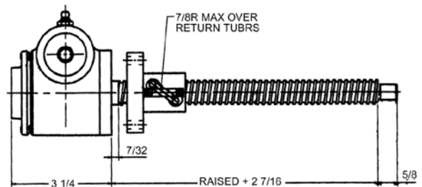
Inverted Rotating: DM-98004
