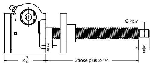
Inverted Rotating: B9250D
