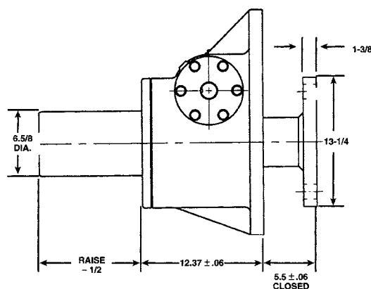
Inverted: M-9074
