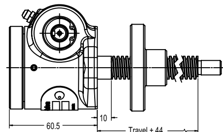
Inverted Rotating: GD2626
