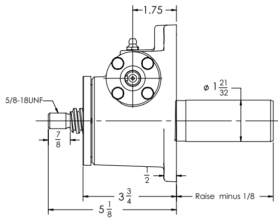
Upright: B9003T
