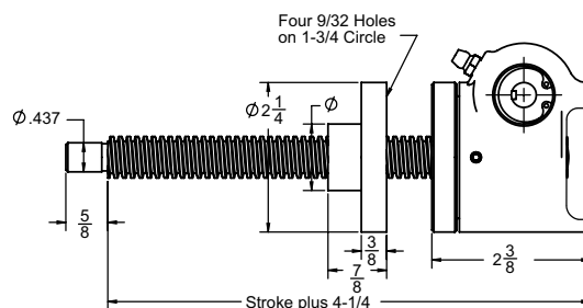
Upright Rotating: B9250U
