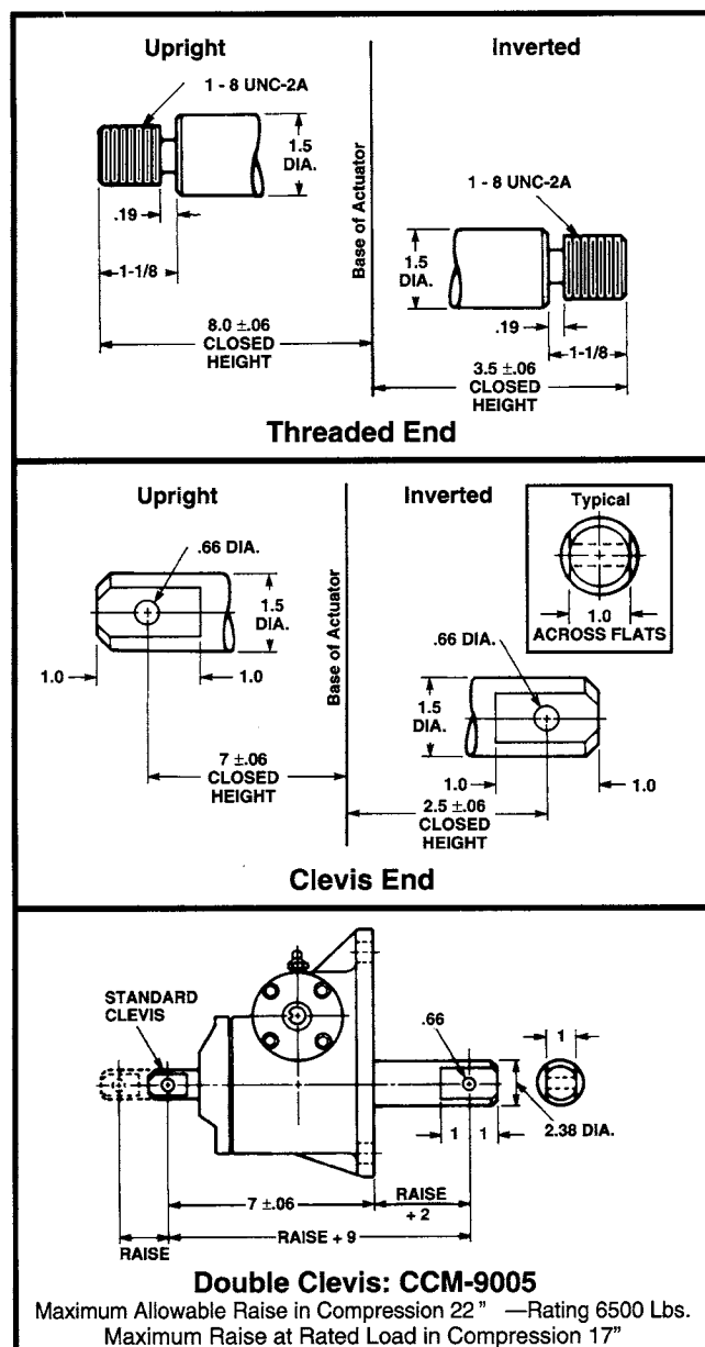
1 1/2" Diameter x .375 Lead Lifting Screws
