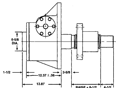
Inverted Rotating: DM-9076
