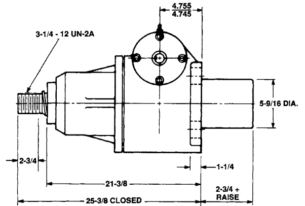
Upright: M-2860
