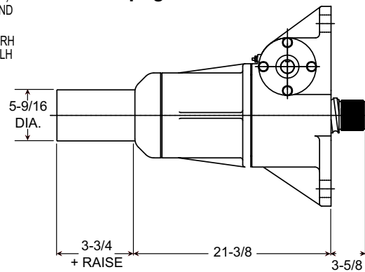
Inverted: M-9859
