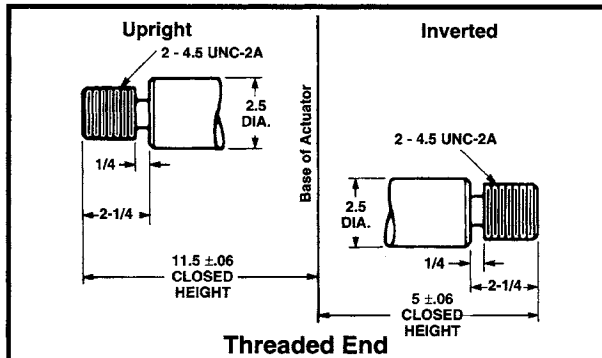
Threaded End
