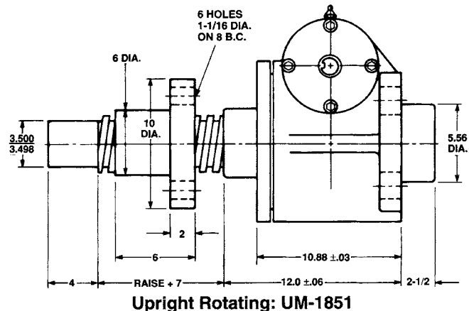
Upright Rotating: UM-1851
