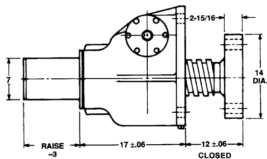
Inverted: M-9098
