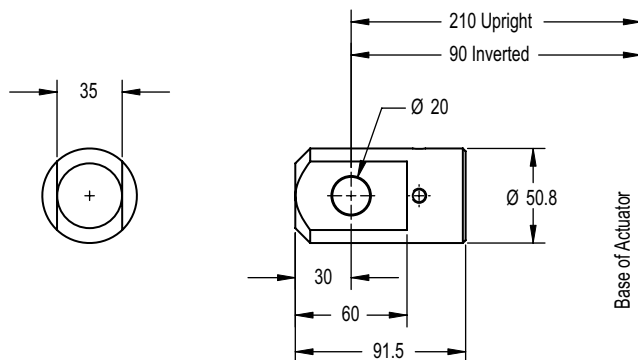
Clevis End G9005-11
