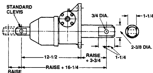
Double Clevis
