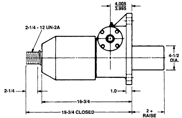
Upright: M-9825
