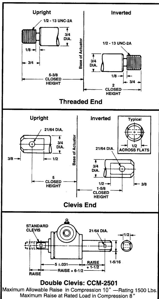
3/4" Diameter x .200 Lead Lifting Screws
