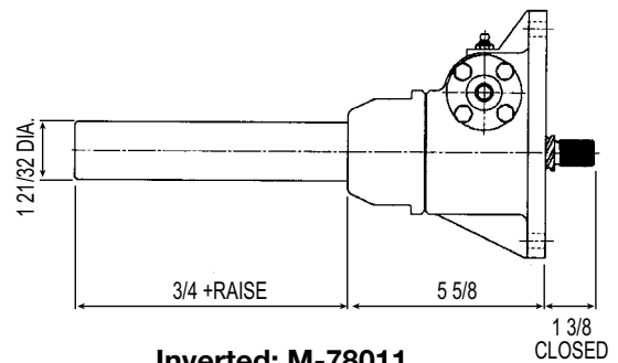
Inverted: M-78011
