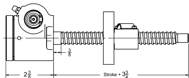
Inverted Rotating: B9863D
