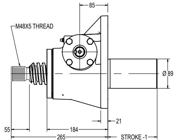
Upright: G9020
