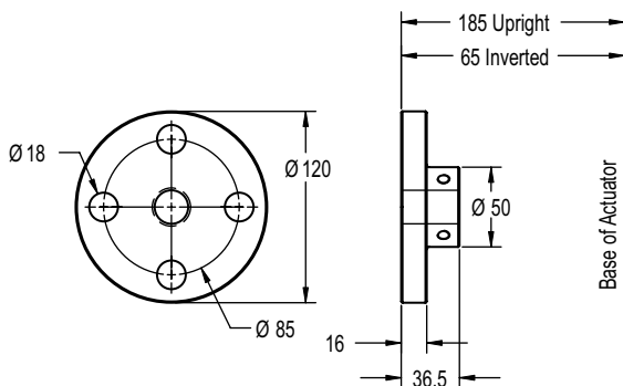
Top Plate G9005-6
