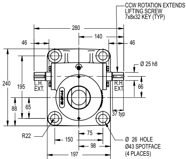
Top View: G9015
