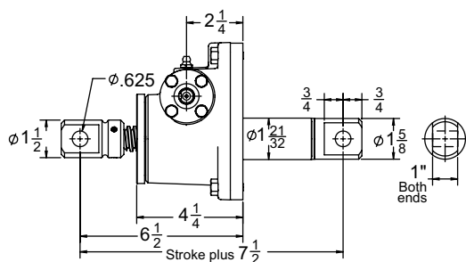
Double Clevis: B9003CC
