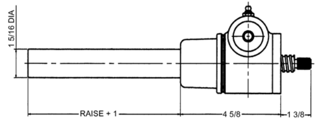
Inverted: M-28749
