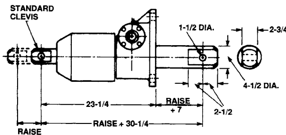
Double Clevis
