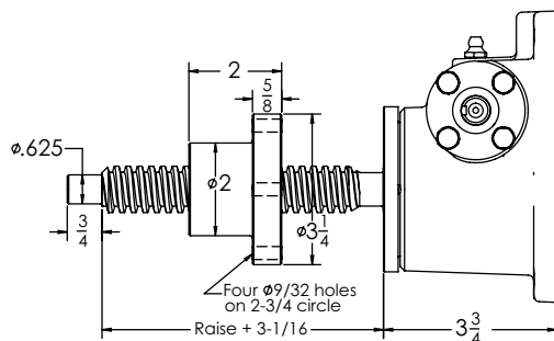
Inverted: B9003TV
