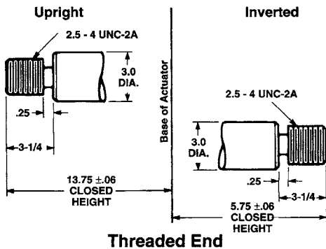
3" Diameter x .666 Lead Lifting Screws
