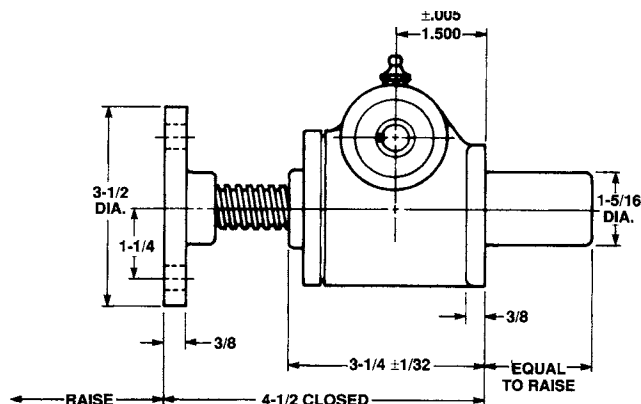
Upright: M-2501
