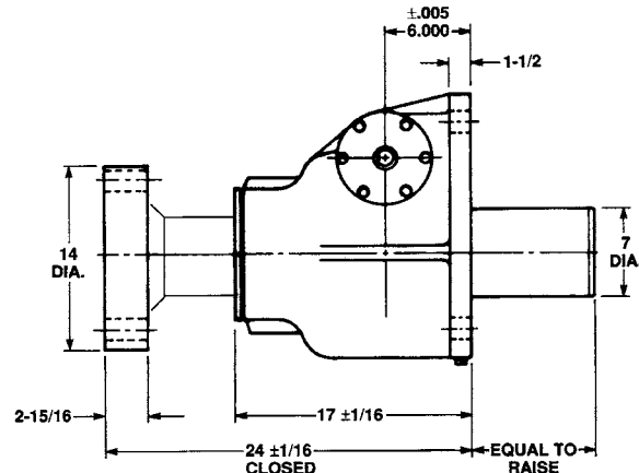
Upright: M-9099
