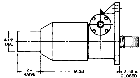
Inverted: M-9824
