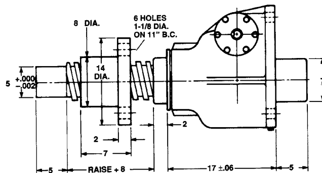
Upright Rotating: UM-9097
