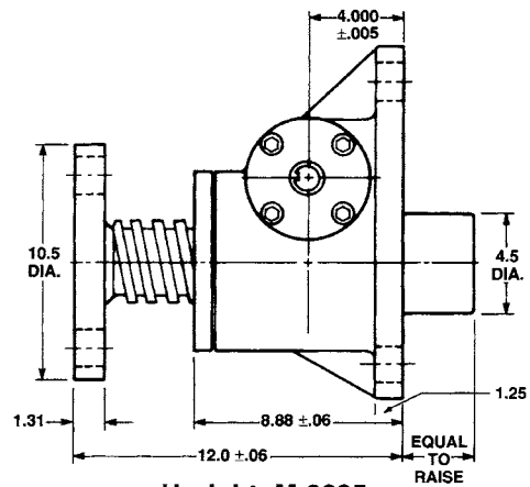
Upright: M-9035
