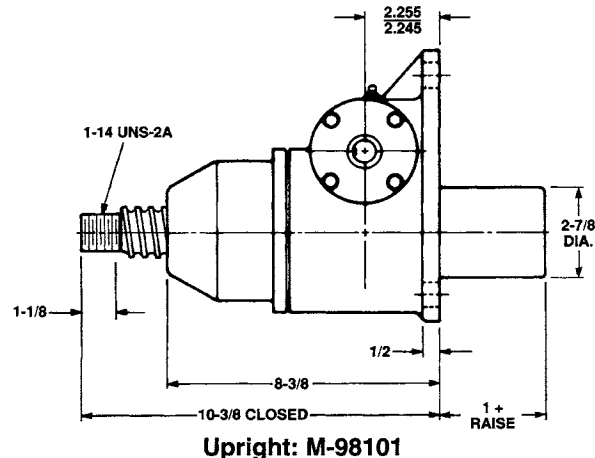
Upright: M-98101
