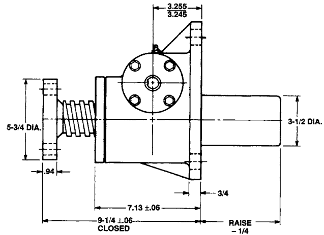
Upright: M-9020
