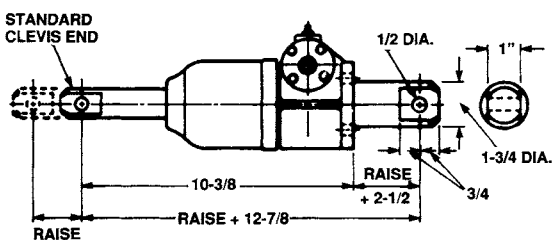
Double Clevis
