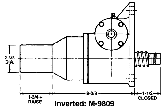
Upright: M-9810
