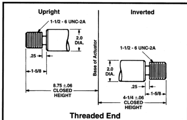
2" Diameter x .500 Lead Lifting Screws
