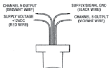
Electrical Connections
