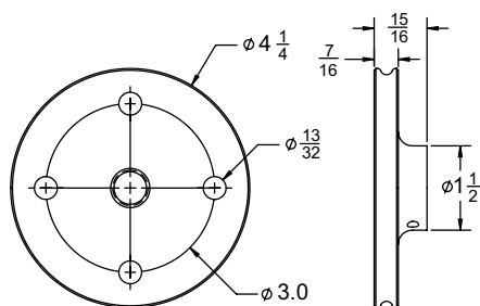
Top Plate SK90003-6A
