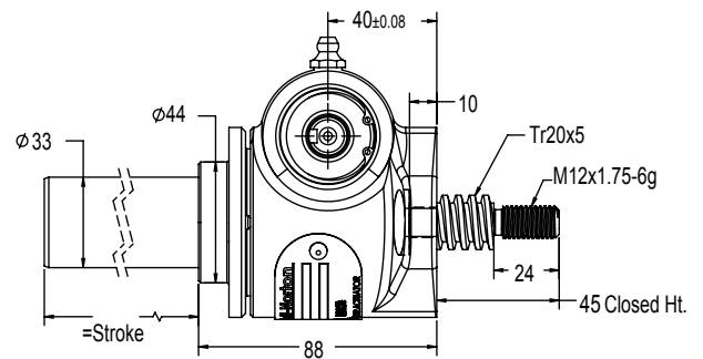
Inverted: G2500
