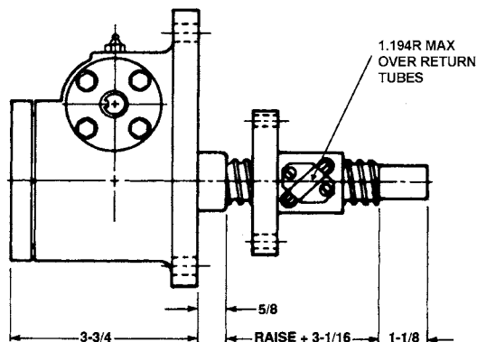
Inverted Rotating: DM-9803
