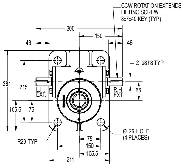
Top View: G9020
