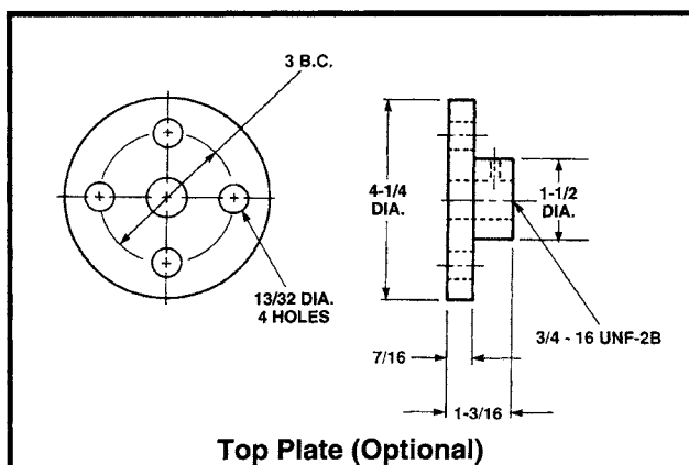
1" Diameter x 1.000 Lead Lifting Screws
