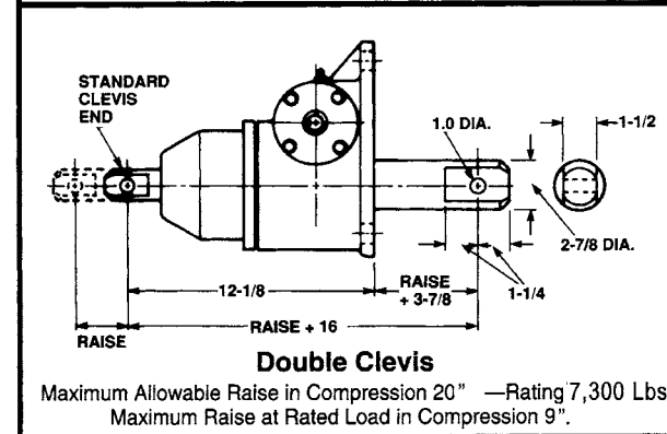
Clevis End (Optional) SK2800-4-10A
